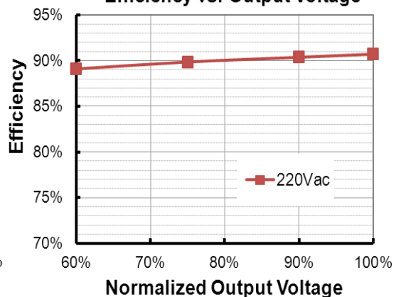
EBD-075S250DV( I_o=2500\text{mA} ) Efficiency vs. Output Voltage
