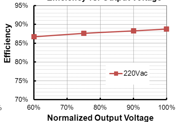
EBD-075S250DV( I_o=2500\text{mA} ) Efficiency vs. Output Voltage
