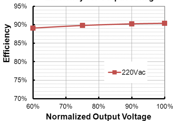
EBD-075S250DV( I_o=1700\text{mA} ) Efficiency vs. Output Voltage
