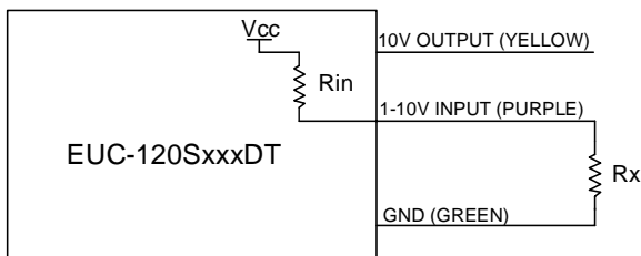
Implementation 2: External resistor (Vcc=12V) 【EUC-120S490DT】
