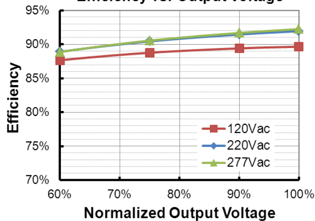
EUD-150S105DTL (I o =1050mA) Efficiency vs. Output Voltage
