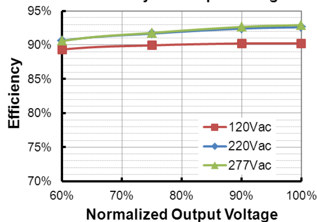
EUD-150S210DTL (I o =1400mA) Efficiency vs. Output Voltage
