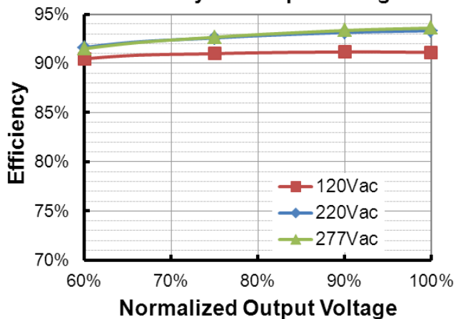
EUD-150S070DTL (I o =450mA) Efficiency vs. Output Voltage
