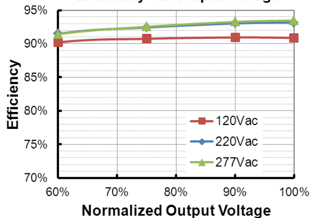
EUD-150S105DTL (I o =700mA) Efficiency vs. Output Voltage
