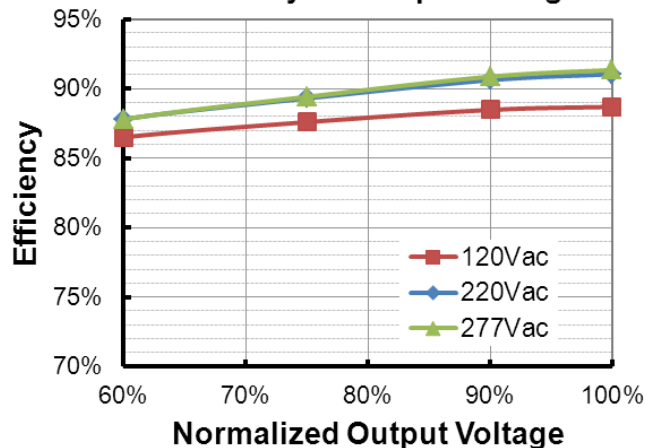
EUD-150S210DTL (I o =2100mA) Efficiency vs. Output Voltage
