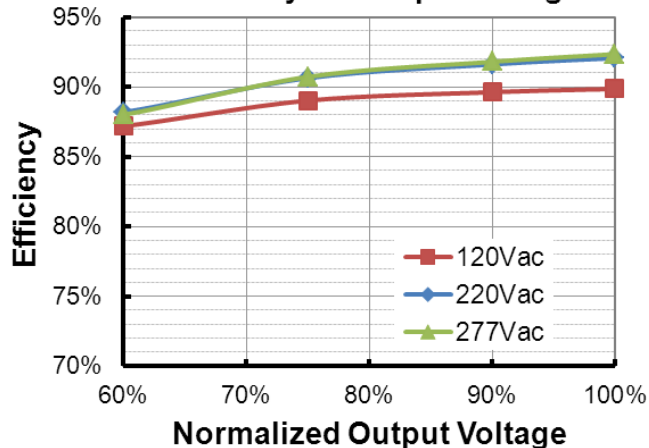
EUD-150S070DTL (I o =700mA) Efficiency vs. Output Voltage
