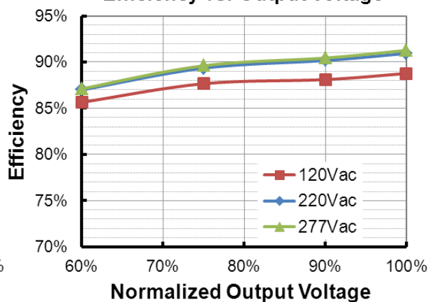
EUD-240S670DTA(I o =6700mA) Efficiency vs. Output Voltage
