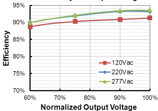
EUD-240S670DTA(I o =4450mA) Efficiency vs. Output Voltage
