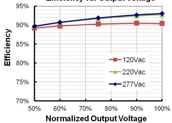
EUD-240S220DV ( I_o=2200mA ) Efficiency vs. Output Voltage
