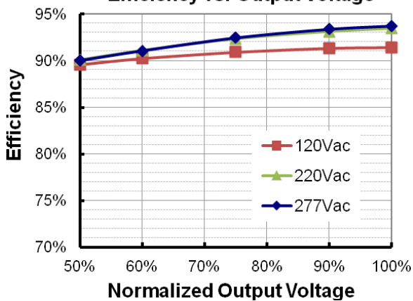
EUD-240S220DV ( I_o=1540mA ) Efficiency vs. Output Voltage
