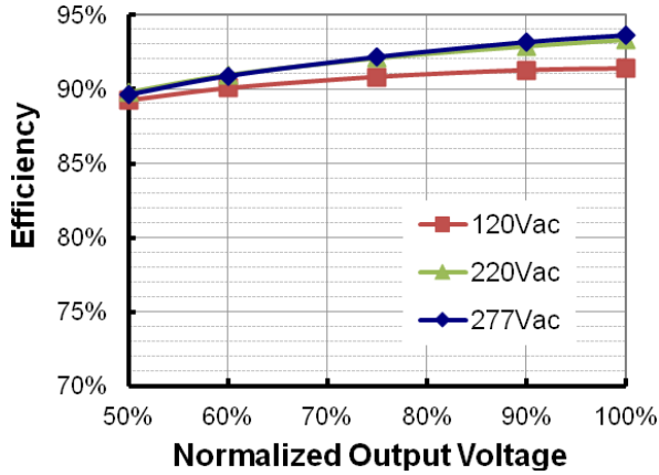
EUD-240S100DV ( I_o=700mA ) Efficiency vs. Output Voltage
