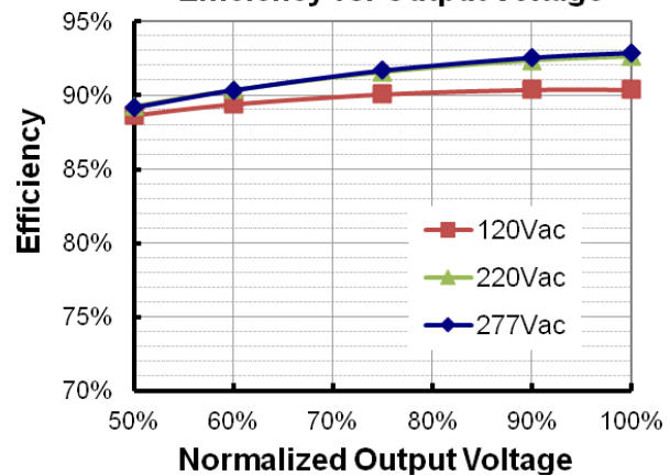
EUD-240S220DV ( I_o=2200mA ) Efficiency vs. Output Voltage
