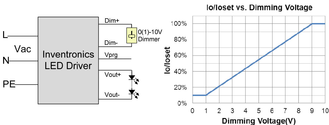
Implementation 1: DC Input
