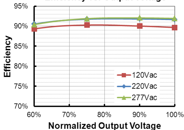
EUR-096S215DT/ST( I_o=1750\text{mA} ) Efficiency vs. Output Voltage
