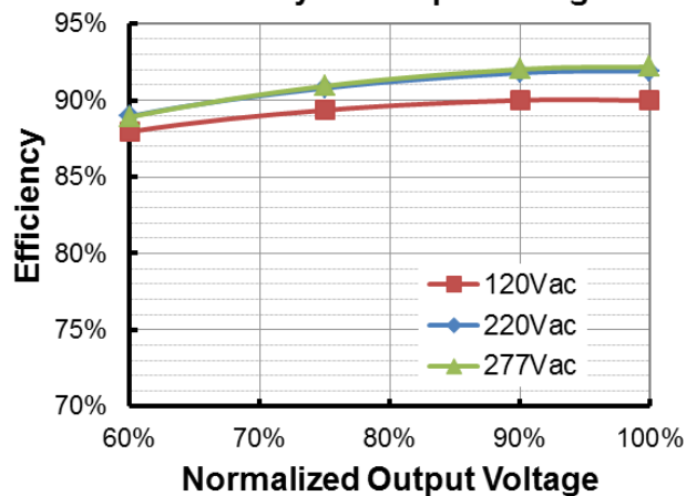
EUR-096S215DT/ST( I_o=1750\text{mA} ) Efficiency vs. Output Voltage
