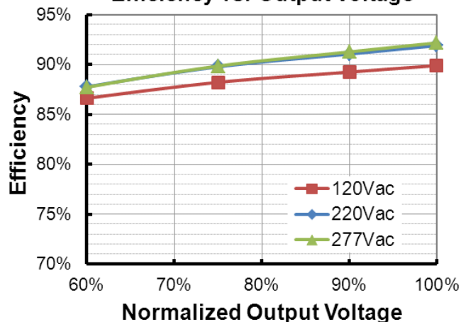
EUR-096S215DT/ST( I_o=2150\text{mA} ) Efficiency vs. Output Voltage
