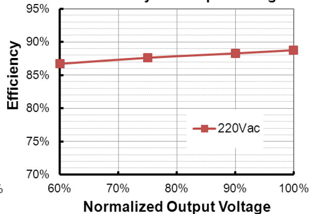
EBD-075S250DV( I_o=2500mA ) Efficiency vs. Output Voltage
