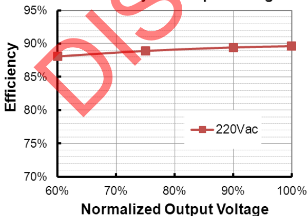
EBD-075S250DV( I_o=1700mA ) Efficiency vs. Output Voltage
