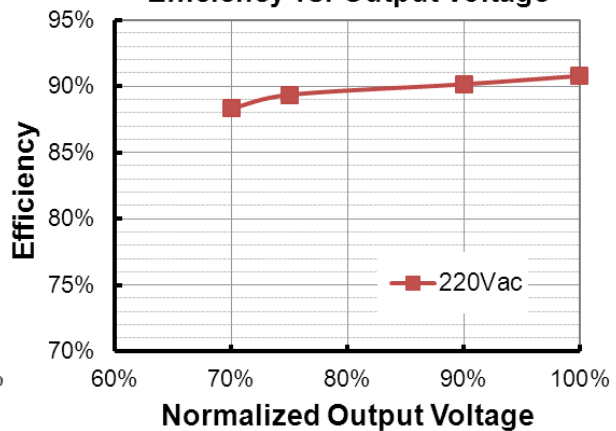
EBD-200S560DV( I_o=5600mA ) Efficiency vs. Output Voltage
