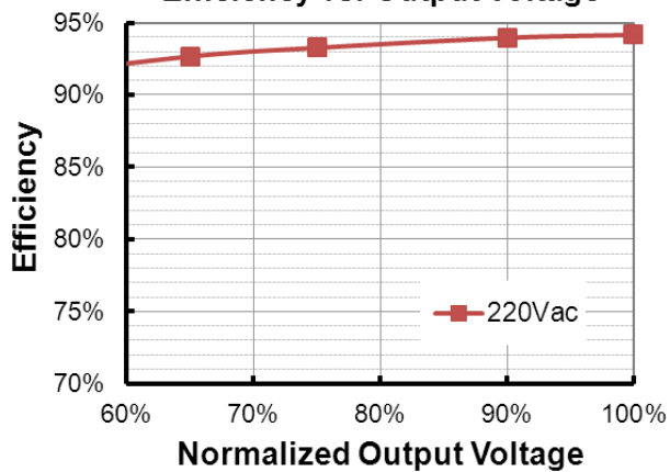
EBD-200S560DV( I_o=3500mA ) Efficiency vs. Output Voltage
