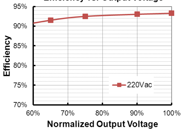
EBD-200S560DV( I_o=3500mA ) Efficiency vs. Output Voltage
