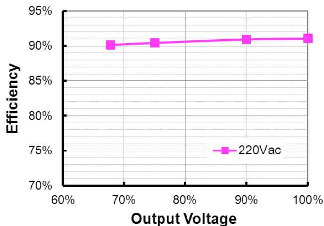
EDC-150S105SV( I_o=1050\text{mA} ) Efficiency vs. Output Voltage
