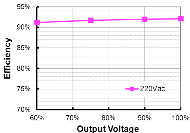
EDC-150S105SV-0004( I_o=860\text{mA} ) Efficiency vs. Output Voltage
