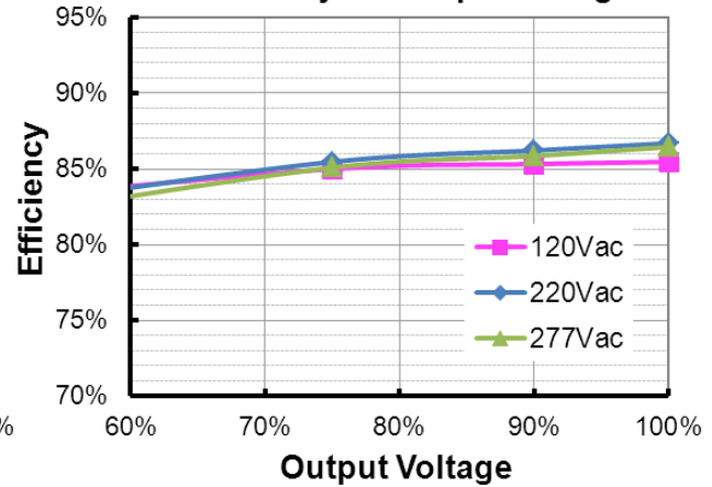
EUC-040S105DVM0004 ( I_o=860mA ) Efficiency vs. Output Voltage
