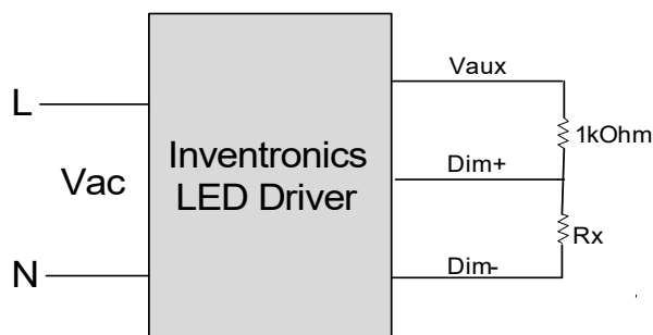
Implementation 2: External Resistor
