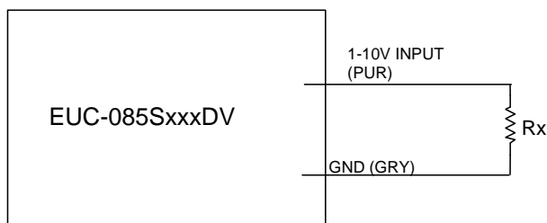
Implementation 2: External resistor
