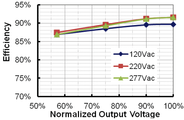
EUC-120T060DV(SV) Efficiency vs. Output Voltage
