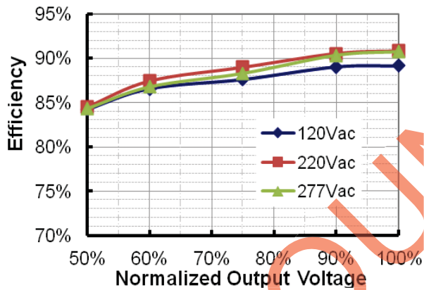
EUC-120T105DV(SV) Efficiency vs. Output Voltage
