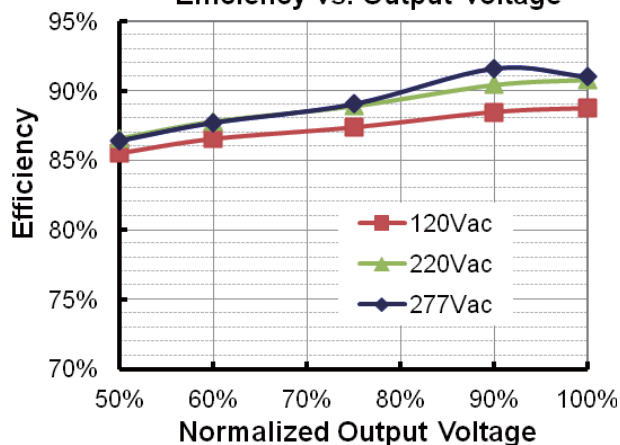
EUC-150S280DVA(SVA) Efficiency vs. Output Voltage
