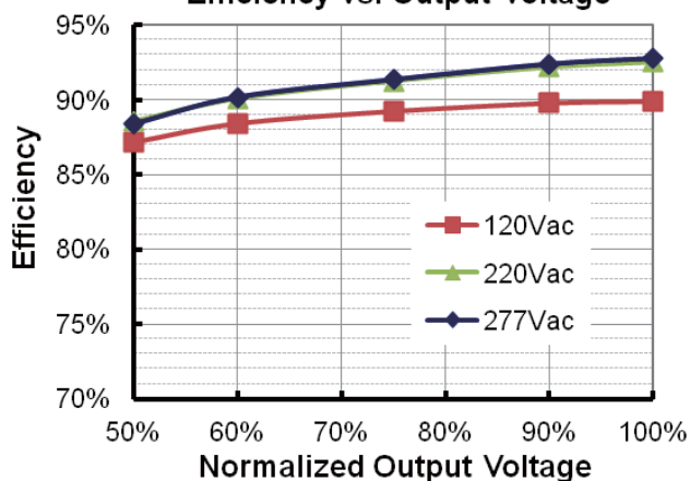
EUC-150S140DVA(SVA) Efficiency vs. Output Voltage
