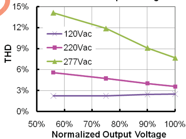
THD vs. Output Voltage
