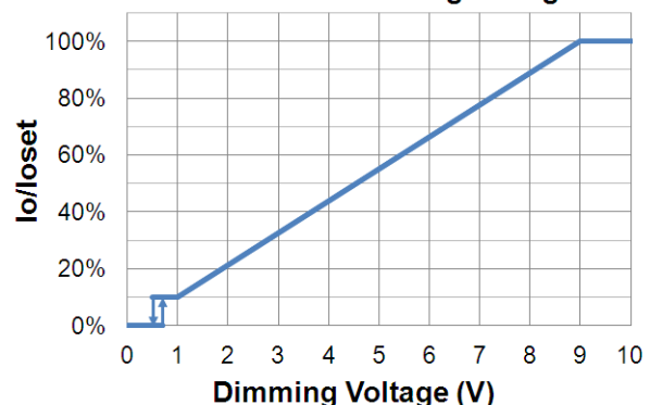
Io/loset vs. Dimming Voltage
