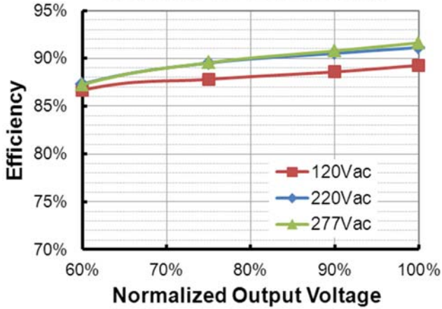
EUD-096S350BTA (I o =2450mA) Efficiency vs. Output Voltage
