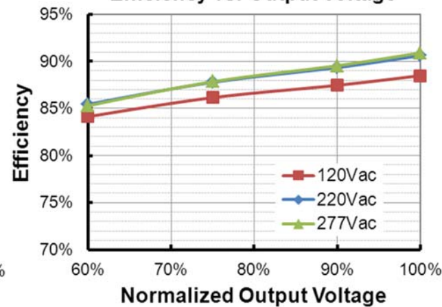
EUD-096S210BVA(I o =2100mA) Efficiency vs. Output Voltage
