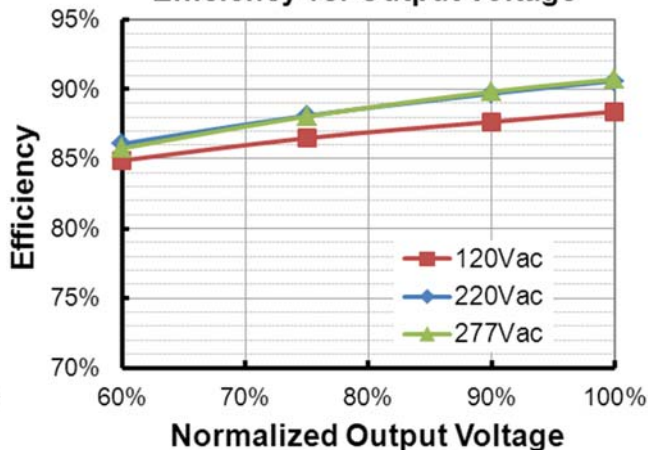
EUD-096S070BVA(I o =700mA) Efficiency vs. Output Voltage
