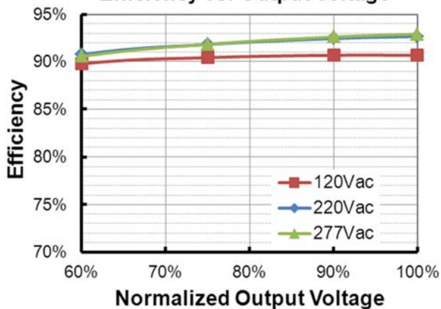
EUD-096S070DVL ( I_o=450\text{mA} ) Efficiency vs. Output Voltage
