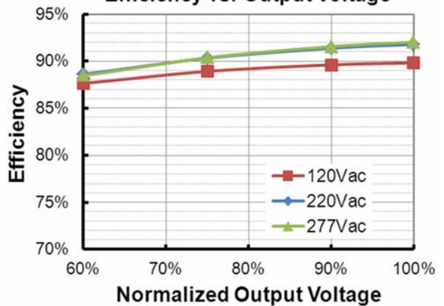
EUD-096S070DVL ( I_o=700\text{mA} ) Efficiency vs. Output Voltage
