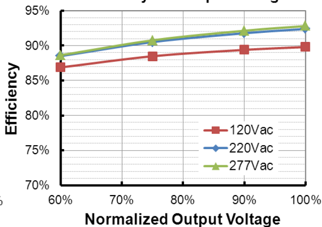
EUD-200S350DVA ( I_o=3500mA ) Efficiency vs. Output Voltage
