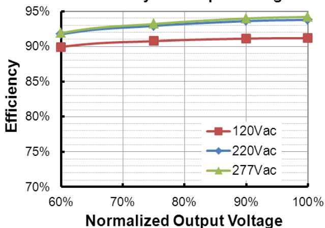
EUD-200S350DVA ( I_o=2450mA ) Efficiency vs. Output Voltage
