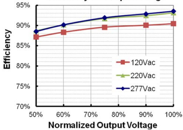
EUD-200S245DV(SV)-00A0 Efficiency vs. Output Voltage
