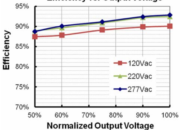
EUD-200S490DV(SV)-00A0 Efficiency vs. Output Voltage
