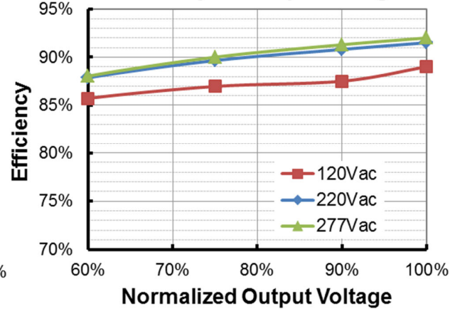
EUD-240S150BVA( I_o=1500mA ) Efficiency vs. Output Voltage
