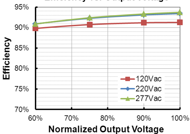
EUD-320S670BT (Io=4690mA) Efficiency vs. Output Voltage
