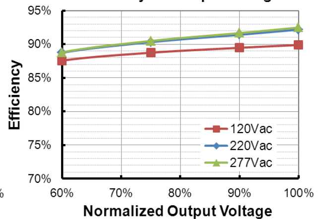
EUD-320S460BT (Io=4600mA) Efficiency vs. Output Voltage
