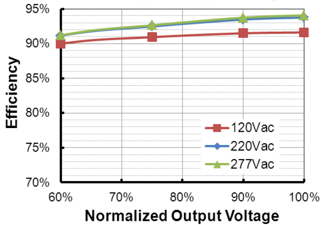
EUD-320S320BT (Io=2240mA) Efficiency vs. Output Voltage
