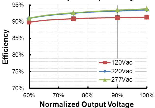
EUD-320S460BT (Io=3220mA) Efficiency vs. Output Voltage
