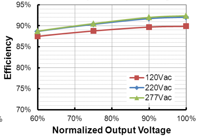
EUD-320S320BT (Io=3200mA) Efficiency vs. Output Voltage
