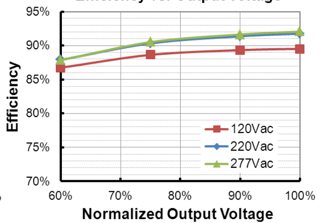
EUD-320S670BT (Io=6700mA) Efficiency vs. Output Voltage
