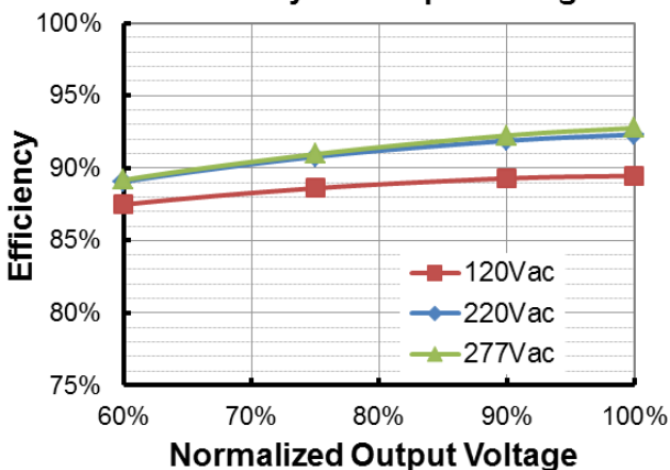
EUK-240S150DT (I o =1500mA) Efficiency vs. Output Voltage
