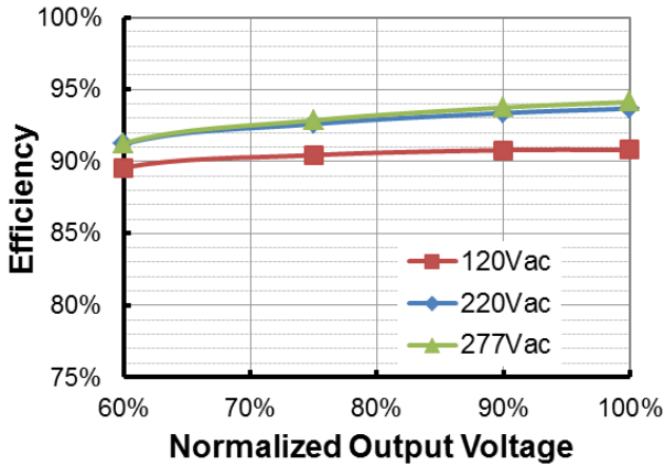
EUK-240S210DT (Io=1400mA) Efficiency vs. Output Voltage
