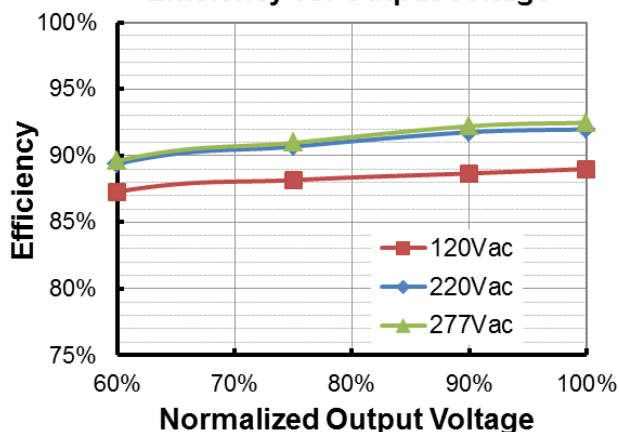
EUK-240S105DT (I o =700mA) Efficiency vs. Output Voltage
