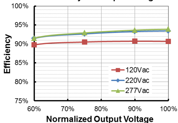
EUK-240S150DT (I o =1050mA) Efficiency vs. Output Voltage
