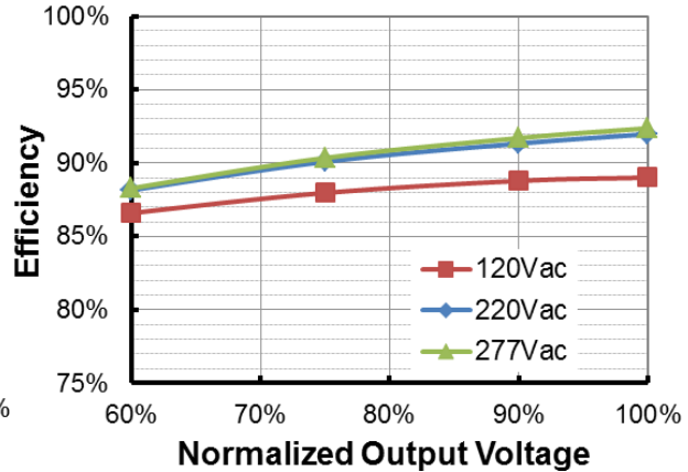
EUK-240S210DT (Io=2100mA) Efficiency vs. Output Voltage
