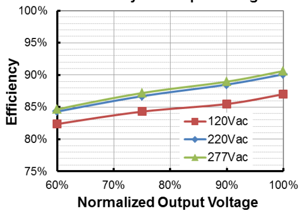
EUK-240S670DT (Io=6700mA) Efficiency vs. Output Voltage
