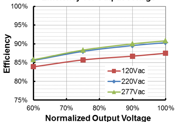
EUK-240S420DT (Io=4200mA) Efficiency vs. Output Voltage
