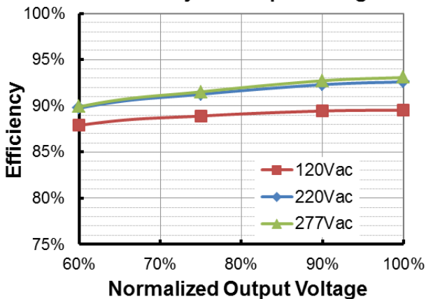
EUK-240S420DT (Io=2800mA) Efficiency vs. Output Voltage
