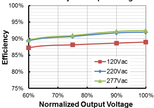
EUK-240S670DT (Io=4600mA) Efficiency vs. Output Voltage
