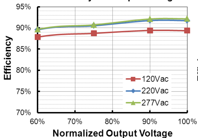
EUR-150S560DV/SV( I_o=3850\text{mA} ) Efficiency vs. Output Voltage
