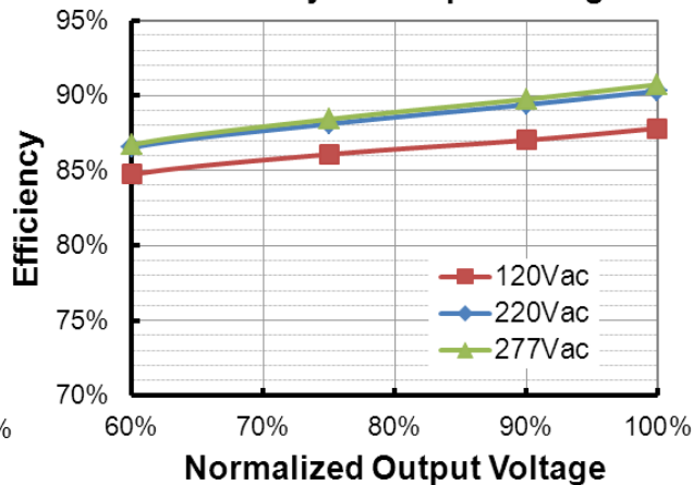
EUR-150S560DV/SV( I_o=5600\text{mA} ) Efficiency vs. Output Voltage
