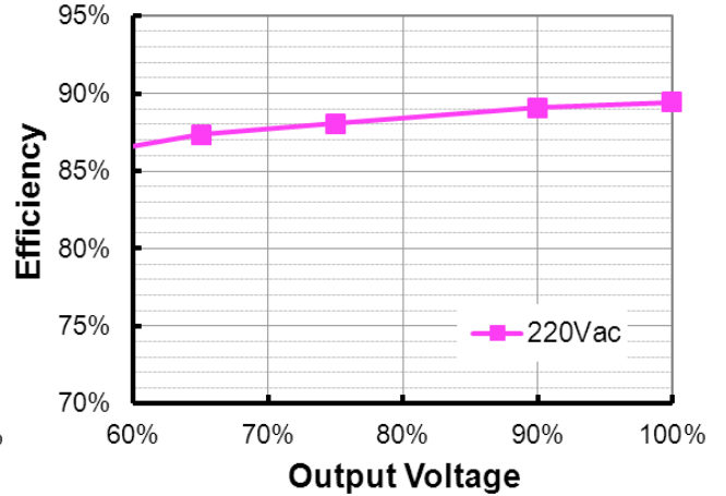
LBD-075S210BSF ( I_o=2100mA ) Efficiency vs. Output Voltage
