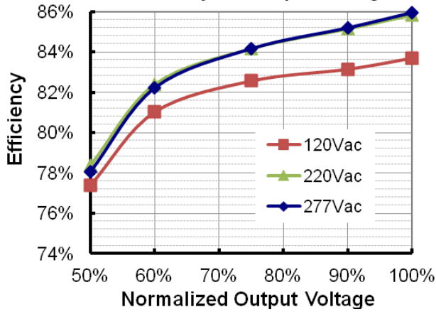
LUC-072Q070DSM(SSM) Efficiency vs. Output Voltage
