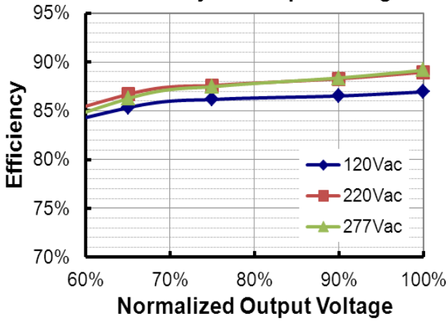
LUD-060S210BS2 (Io=1470mA) Efficiency vs. Output Voltage
