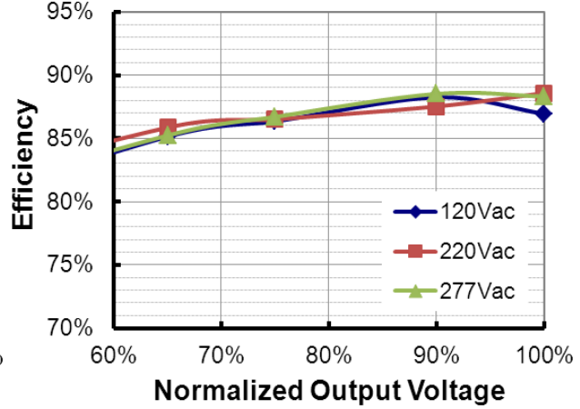
LUD-060S210BS2 (Io=2100mA) Efficiency vs. Output Voltage
