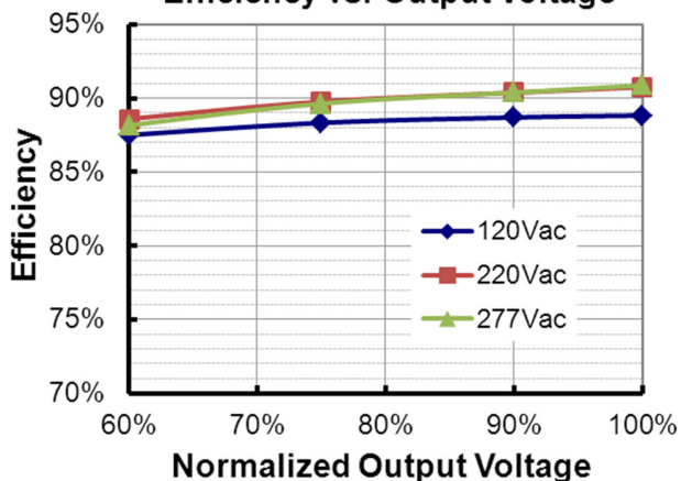
LUD-060S110DS2( I_o=770\text{mA} ) Efficiency vs. Output Voltage
