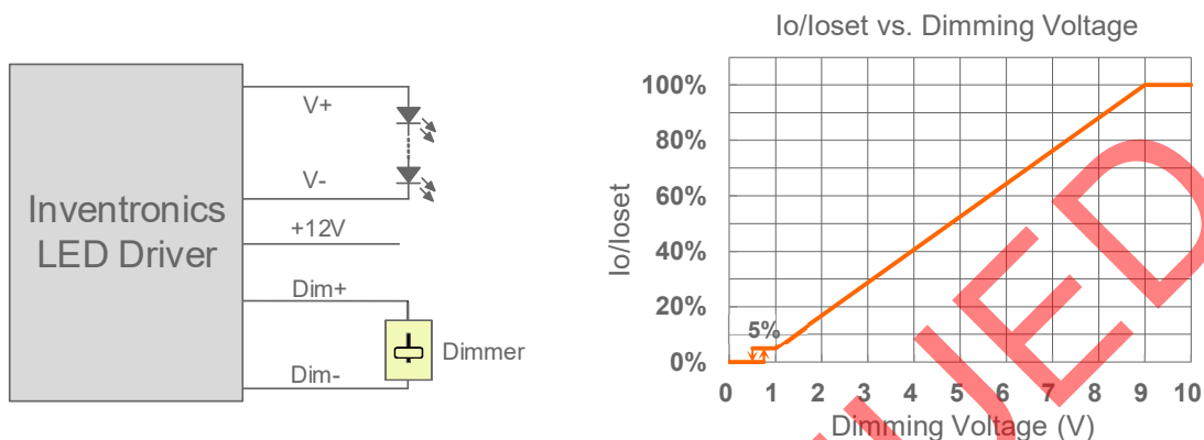
Implementation 1: DC Input
