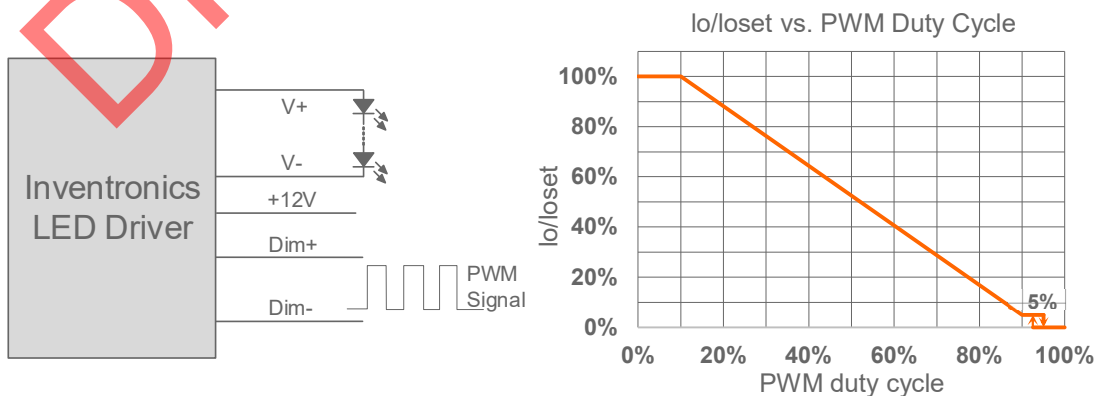
Implementation 3: Negative logic
