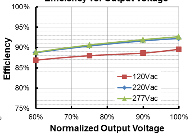
EUK-240S150DT(TT)( I_o=1500mA ) Efficiency vs. Output Voltage
