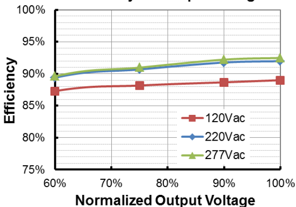
EUK-240S670DT(TT)(I o =4600mA) Efficiency vs. Output Voltage
