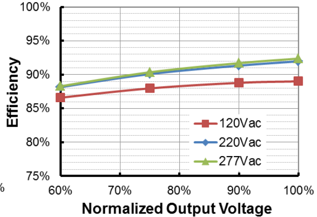
EUK-240S210DT(TT)(I o =2100mA) Efficiency vs. Output Voltage
