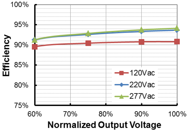
EUK-240S210DT(TT)(I o =1400mA) Efficiency vs. Output Voltage
