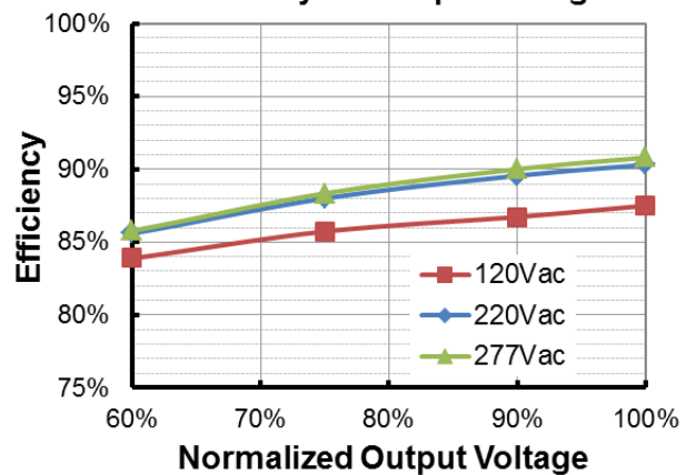
EUK-240S420DT(TT)(I o =4200mA) Efficiency vs. Output Voltage
