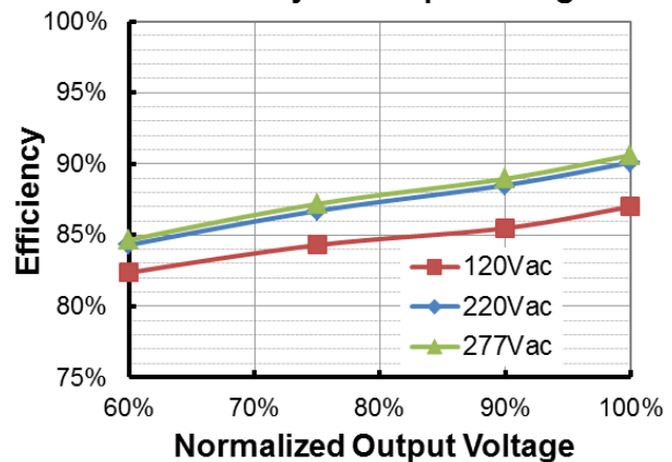
EUK-240S670DT(TT)(I o =6700mA) Efficiency vs. Output Voltage
