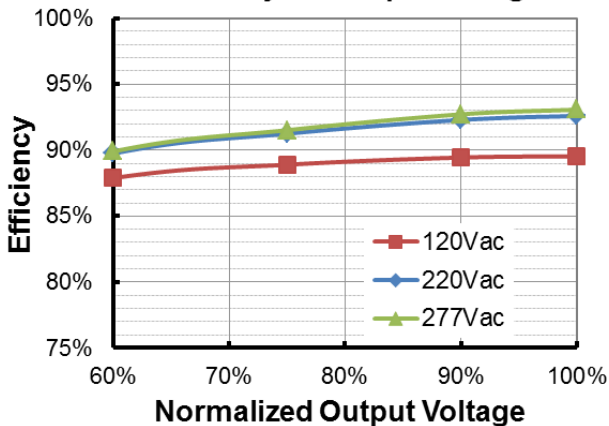
EUK-240S420DT(TT)(I o =2800mA) Efficiency vs. Output Voltage
