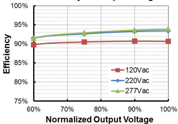
EUK-240S150DT(TT)( I_o=1050mA ) Efficiency vs. Output Voltage
