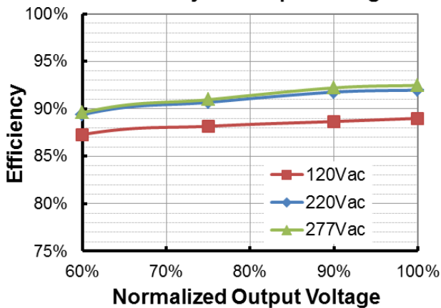
EUK-240S105DT(TT)( I_o=700mA ) Efficiency vs. Output Voltage
