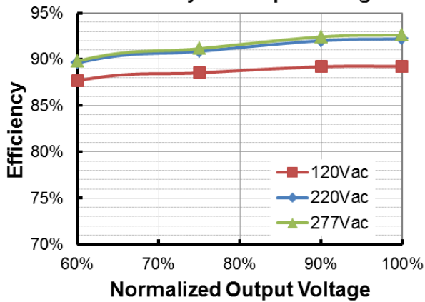
HUK-200S560DT( I_o=3850\text{mA} ) Efficiency vs. Output Voltage
