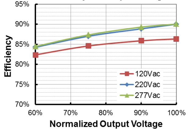
HUK-200S560DT( I_o=5600\text{mA} ) Efficiency vs. Output Voltage
