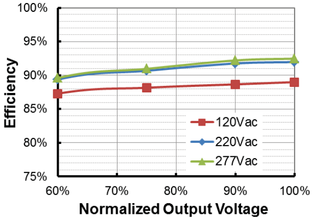
HUK-240S670DT (Io=4600mA) Efficiency vs. Output Voltage
