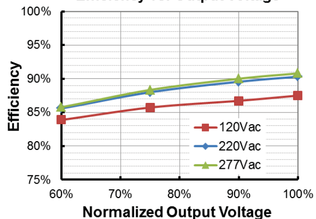
HUK-240S420DT (I o =4200mA) Efficiency vs. Output Voltage
