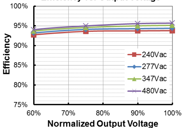
EFD-1K2S420DV (Io=3360mA) Efficiency vs. Output Voltage
