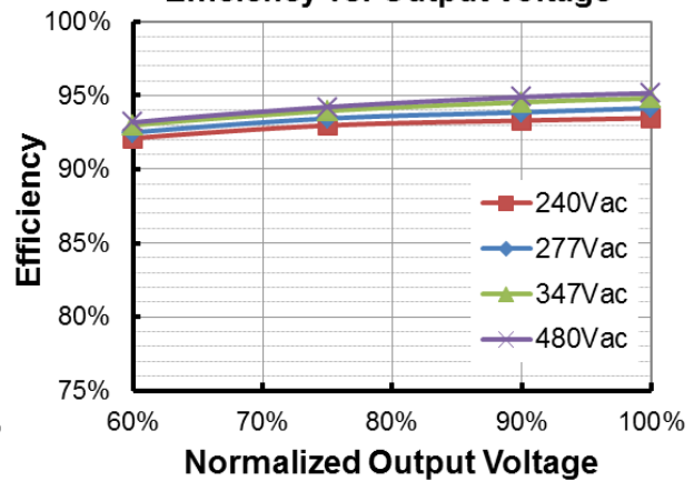
EFD-1K2S420DV (Io=4200mA) Efficiency vs. Output Voltage
