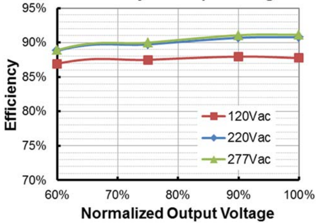
EUG-192D400DT (I o =2650mA) Efficiency vs. Output Voltage
