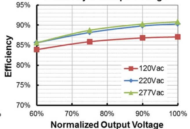
EUG-192D265DT (I o =2650mA) Efficiency vs. Output Voltage
