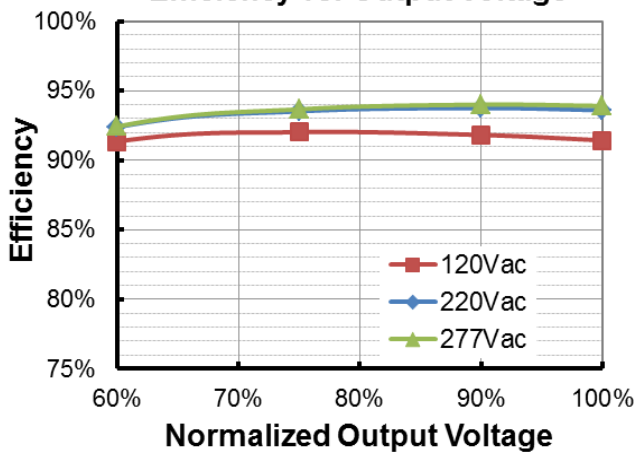
EUK-320S150DV(TV)( I_o=1050mA ) Efficiency vs. Output Voltage
