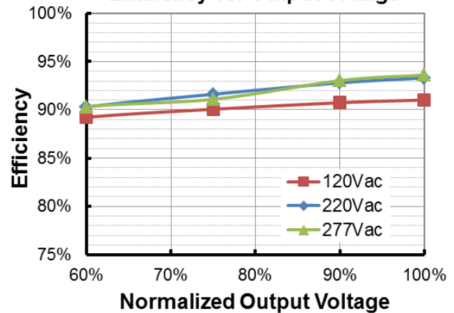
EUK-320S220DV(TV)( I_o=2200mA ) Efficiency vs. Output Voltage
