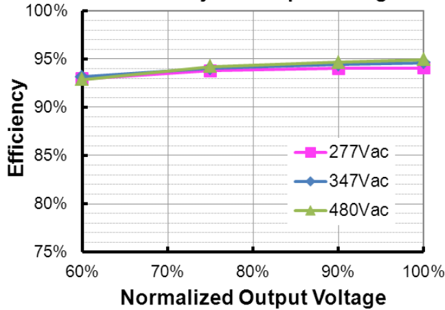
ESD-480S140DT (Io=1050mA) Efficiency vs. Output Voltage
