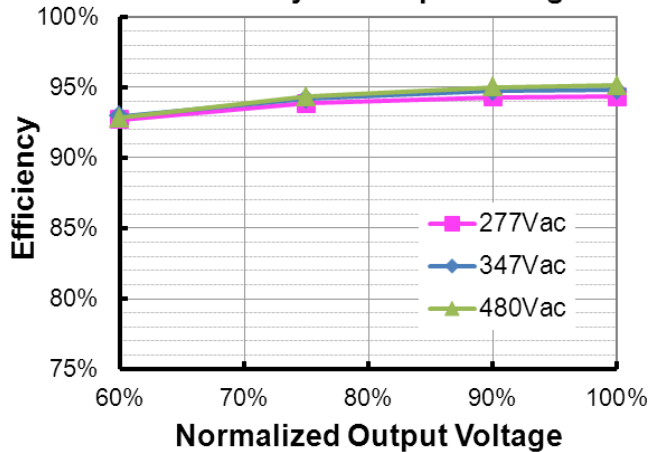
ESD-480S420DT (Io=3150mA) Efficiency vs. Output Voltage
