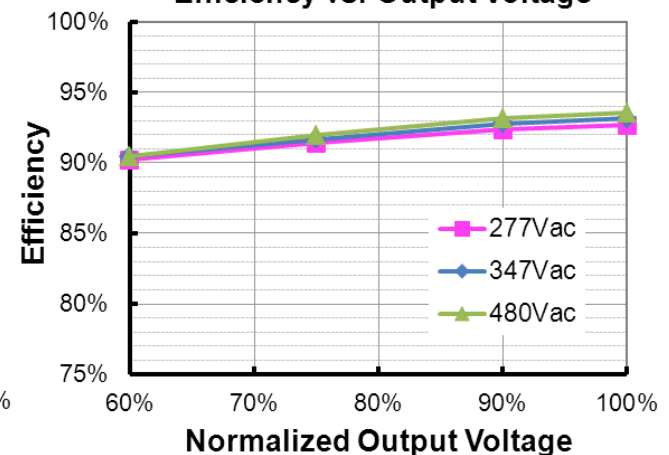
ESD-480S420DT (Io=4200mA) Efficiency vs. Output Voltage
