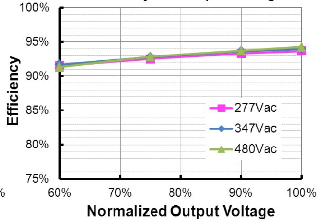
ESD-480S140DT (Io=1400mA) Efficiency vs. Output Voltage
