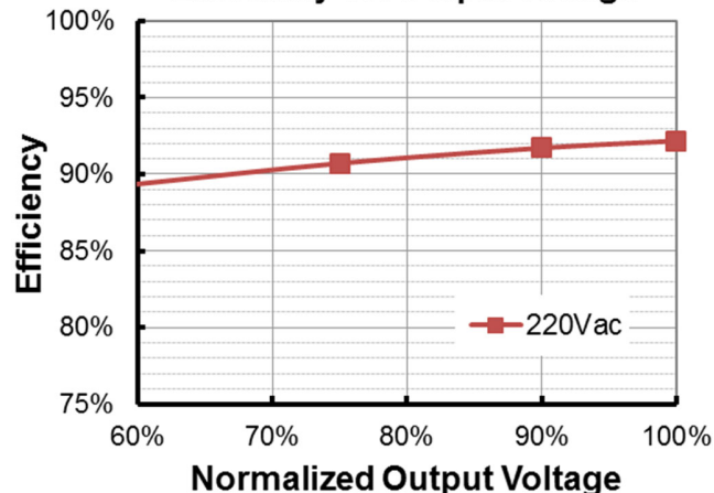
LMT-080S105STF( I_o=1050mA ) Efficiency vs. Output Voltage
