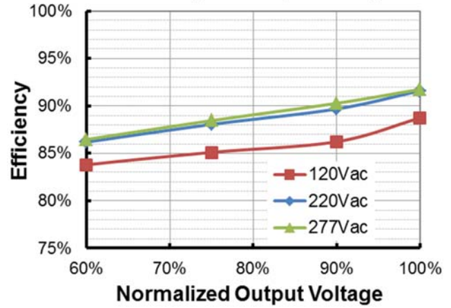
EUP-320S670SV (Io=6700mA) Efficiency vs. Output Voltage
