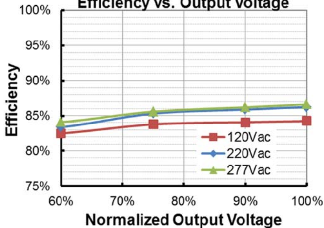
LUN-042S150DT(ST)( I_o=1500\text{mA} ) Efficiency vs. Output Voltage
