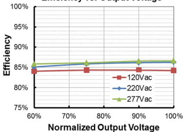
LUN-042S150DT(ST)( I_o=1050\text{mA} ) Efficiency vs. Output Voltage
