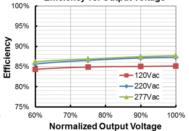
LUN-042S105DT(ST) (Io=1050mA) Efficiency vs. Output Voltage
