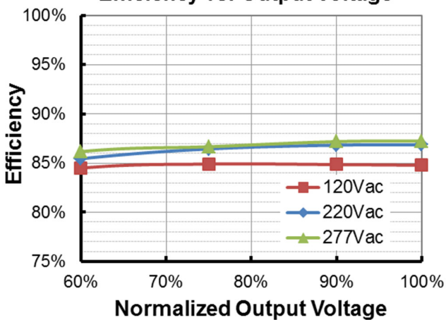
LUN-042S105DT(ST) (Io=780mA) Efficiency vs. Output Voltage
