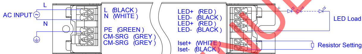
Wire Connection 1
