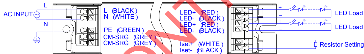
Wire Connection 2
