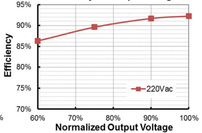
EBS-080S150BT2 (Io=1500mA) Efficiency vs. Output Voltage
