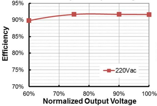
EBS-080S150BT2 (Io=1050mA) Efficiency vs. Output Voltage
