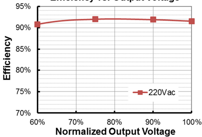
EBS-080S105BT2( I_o=700 mA) Efficiency vs. Output Voltage
