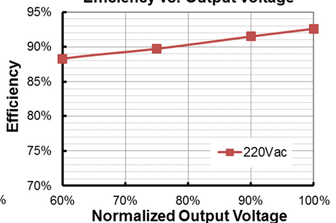
EBS-080S105BT2( I_o=1050 mA) Efficiency vs. Output Voltage
