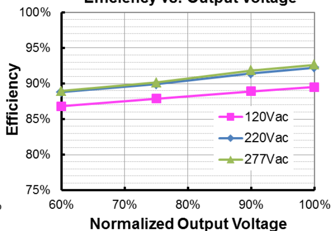
EUM-240S670Bx ( I_o=6700\text{mA} ) Efficiency vs. Output Voltage
