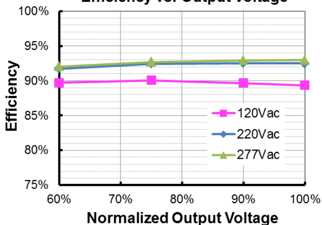
EUM-240S670Bx ( I_o=4200\text{mA} ) Efficiency vs. Output Voltage
