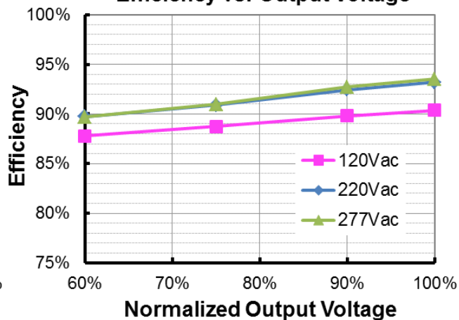
EUM-240S350Bx ( I_o=3500\text{mA} ) Efficiency vs. Output Voltage
