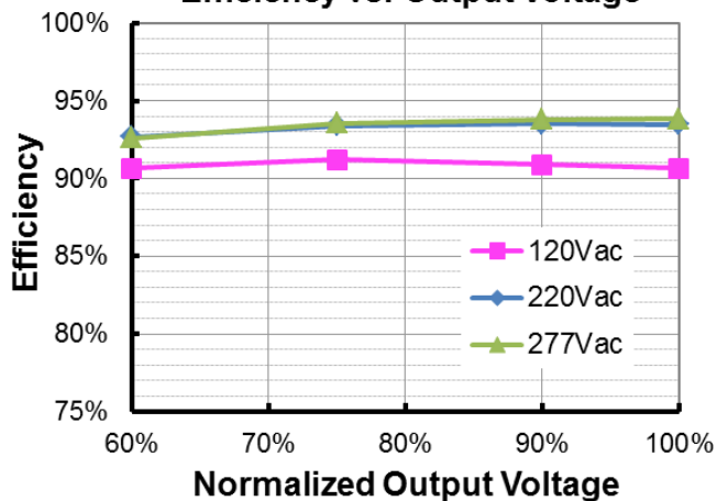
EUM-240S350Bx ( I_o=2150\text{mA} ) Efficiency vs. Output Voltage
