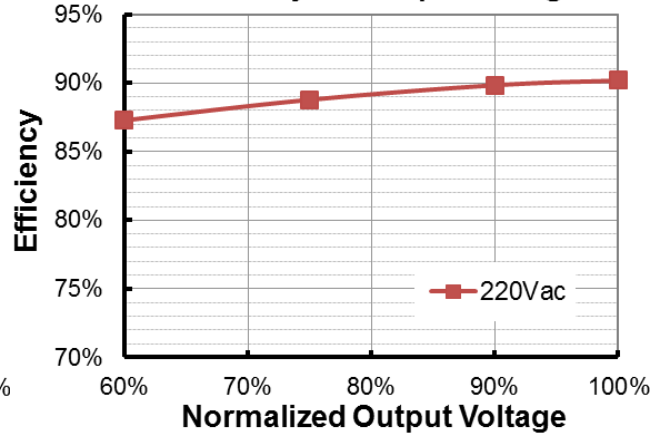
EBS-040S070BT2 (I o =700mA) Efficiency vs. Output Voltage
