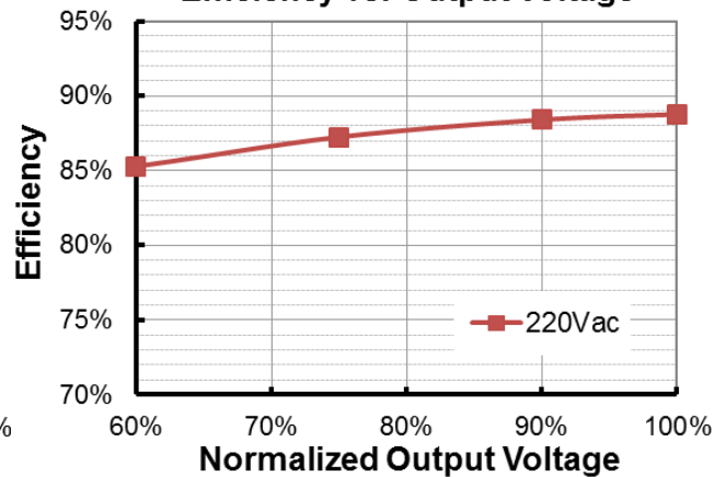
EBS-040S105BT2 (I o =1050mA) Efficiency vs. Output Voltage
