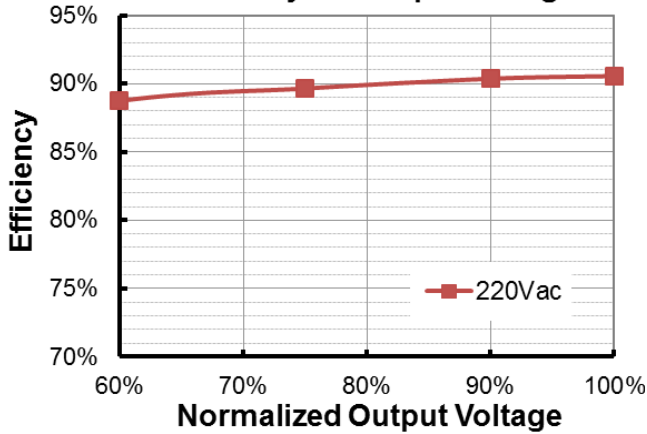
EBS-040S045BT2 (I o =300mA) Efficiency vs. Output Voltage
