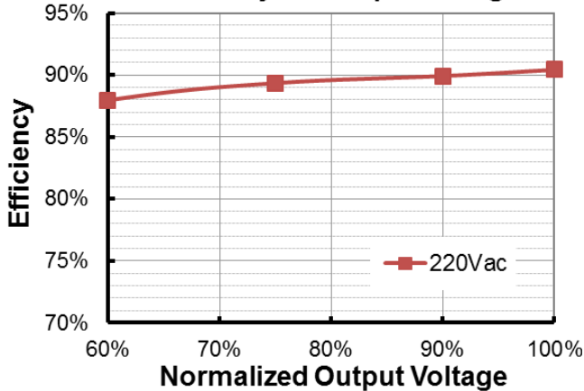
EBS-040S070BT2 (I o =450mA) Efficiency vs. Output Voltage
