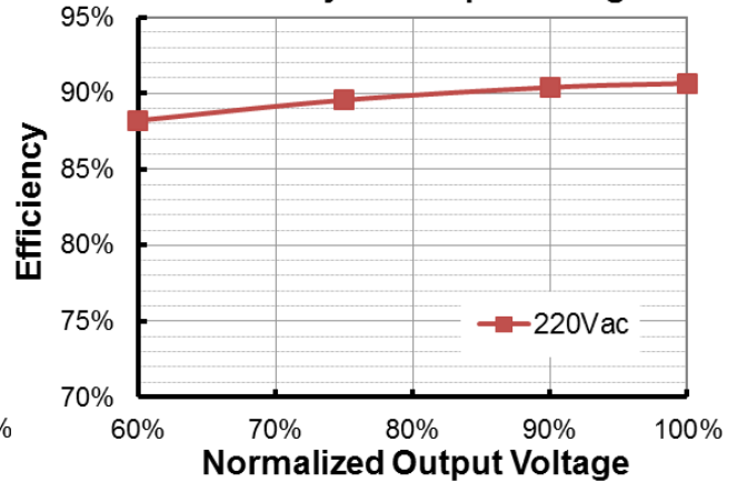
EBS-040S045BT2 (I o =450mA) Efficiency vs. Output Voltage
