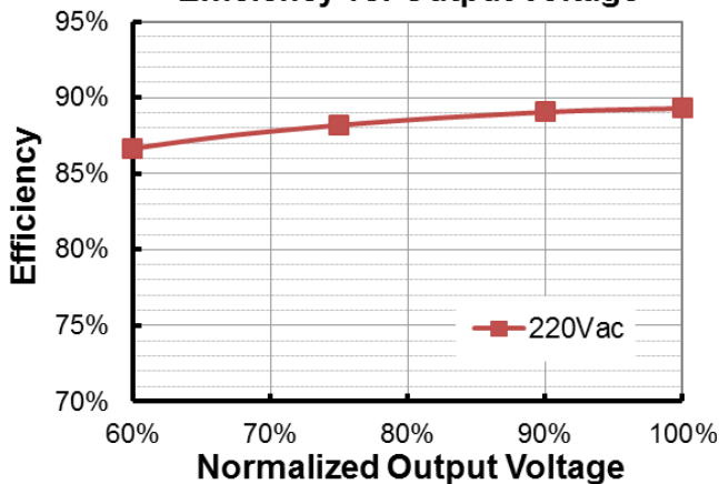
EBS-040S105BT2 (I o =700mA) Efficiency vs. Output Voltage
