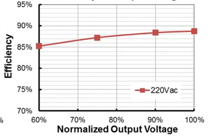
EBS-040S105BT2 (Io=1050mA) Efficiency vs. Output Voltage
