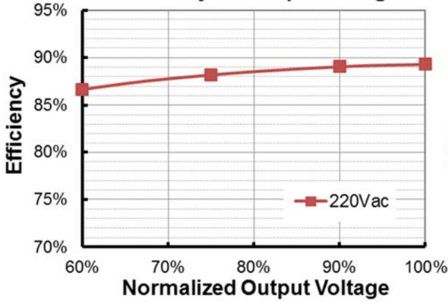
EBS-040S105BT2 (Io=700mA) Efficiency vs. Output Voltage
