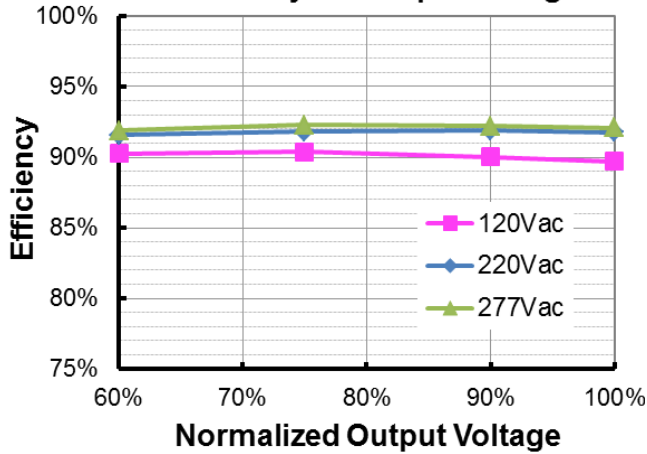
EUM-100S280Bx( I_o=1750\text{mA} ) Efficiency vs. Output Voltage
