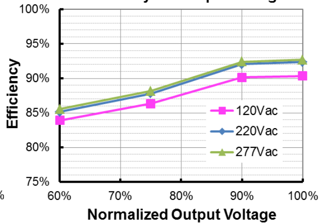
EUM-100S280Bx( I_o=2800\text{mA} ) Efficiency vs. Output Voltage
