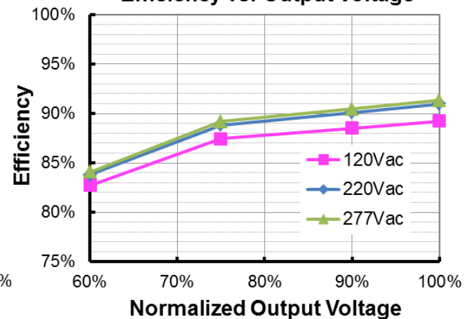
EUM-100S280Bx( I_o=2800\text{mA} ) Efficiency vs. Output Voltage
