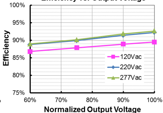
EUM-240S350Mx ( I_o=3500\text{mA} ) Efficiency vs. Output Voltage
