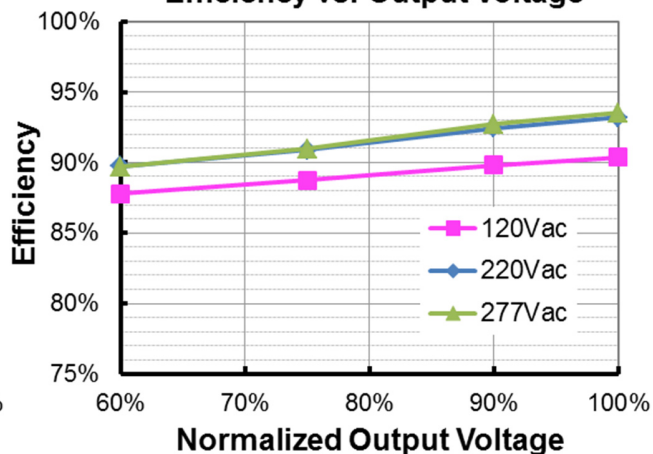
EUM-240S150Mx ( I_o=1500\text{mA} ) Efficiency vs. Output Voltage
