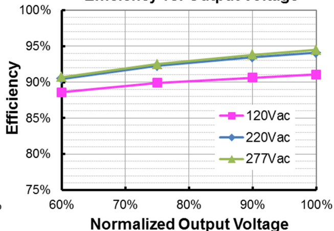
EUM-240S105Mx ( I_o=1050\text{mA} ) Efficiency vs. Output Voltage
