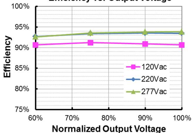
EUM-240S150Mx ( I_o=1050\text{mA} ) Efficiency vs. Output Voltage
