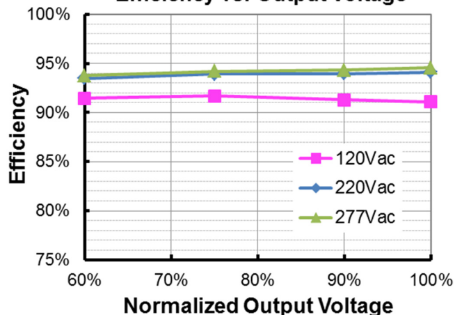
EUM-240S105Mx ( I_o=700\text{mA} ) Efficiency vs. Output Voltage
