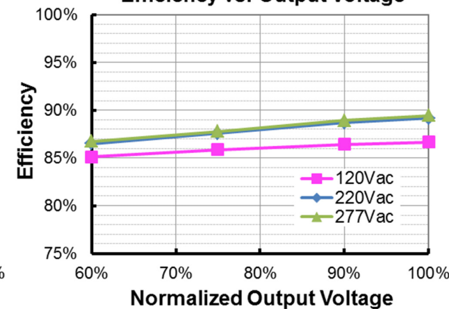
EUM-075S150Mx ( I_o=1500mA )
