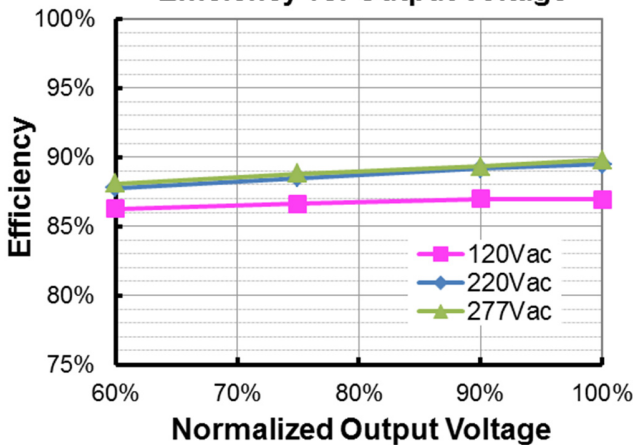
EUM-075S150Mx ( I_o=1050mA )
