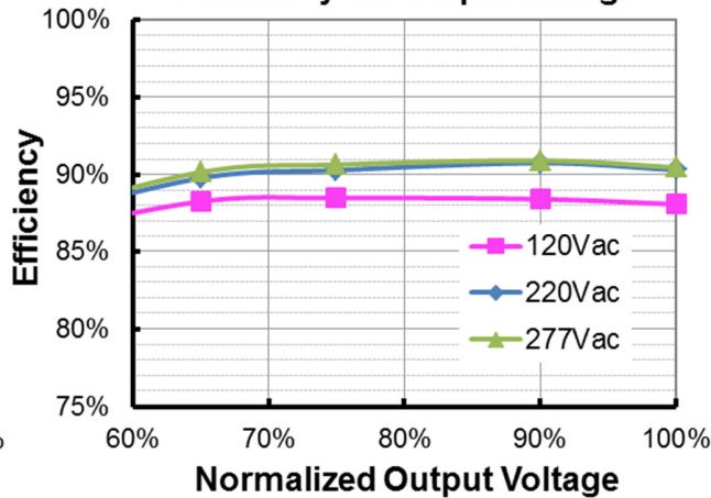
EUM-075S150Mx ( I_o=1500mA )
